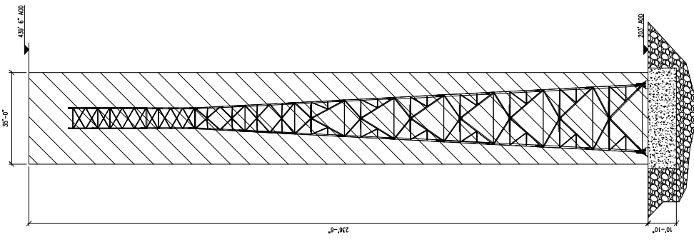
2. TOWER ELEVATION AND ENVELOPE SCALE: 1/16" = 1'-0"
