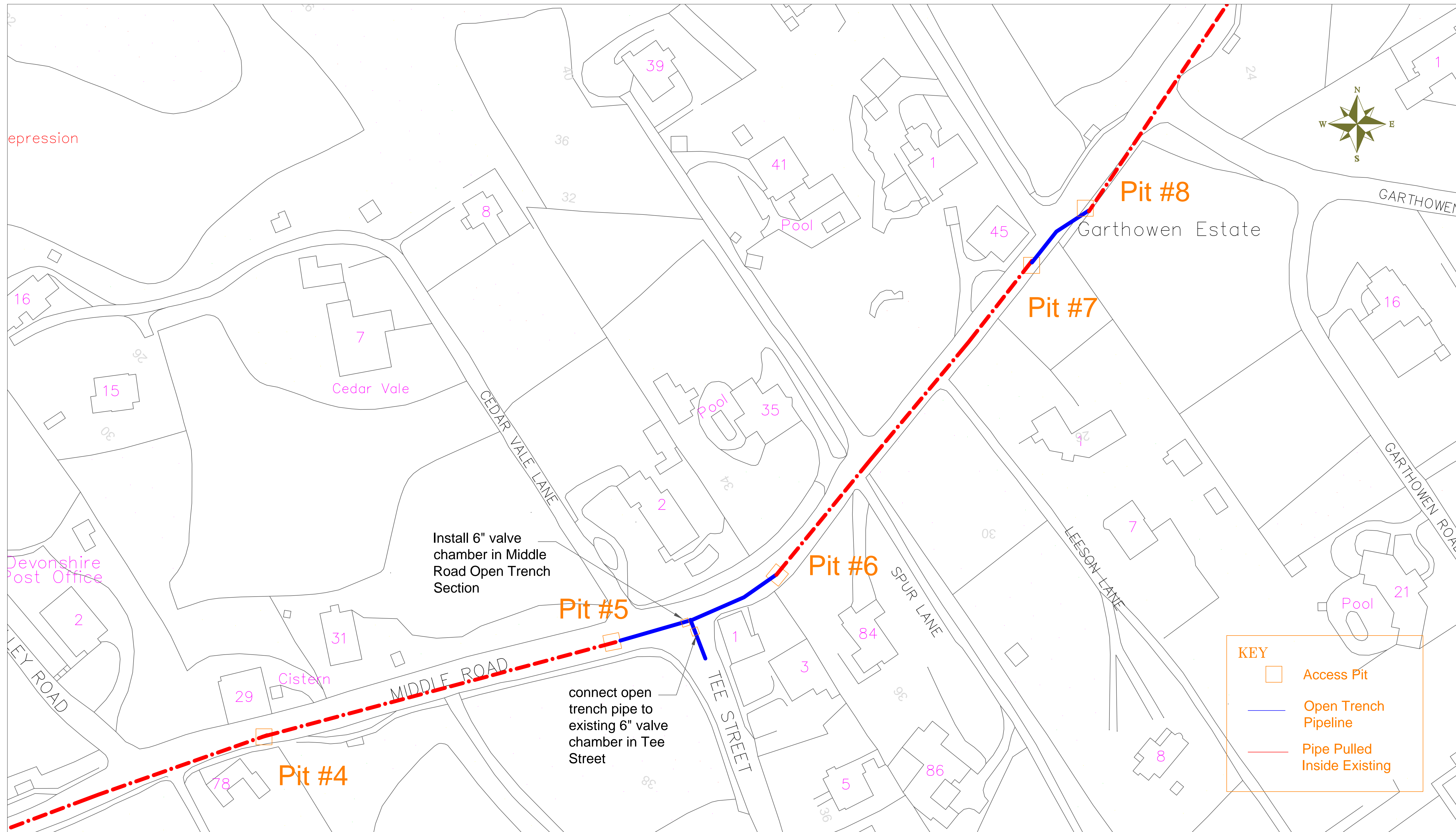
PIPELINE PLAN 1-500
