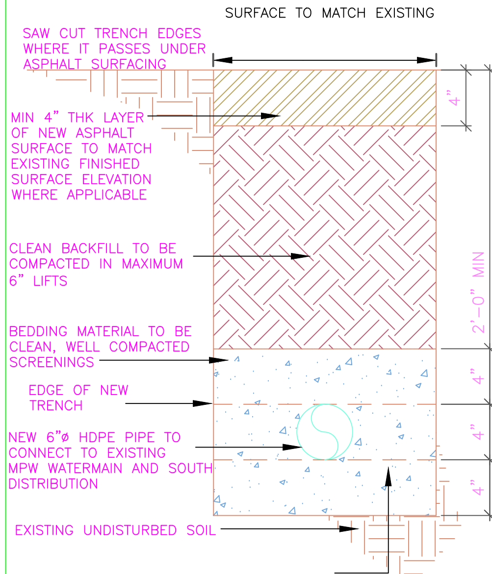
CROSS-SECTION OF NEW TRENCH N.T.S.
